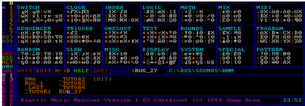
Figure 14. KMM menus
